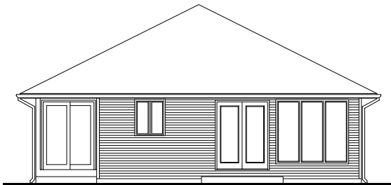
NORTH ELEVATION
