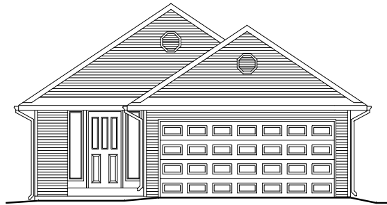
SOUTH ELEVATION
